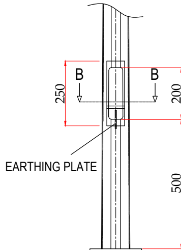
FUSE DETAIL
