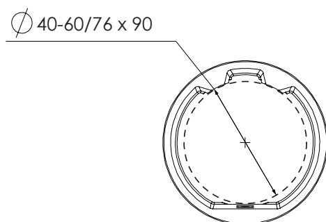
Dimensions with NEMA socket
