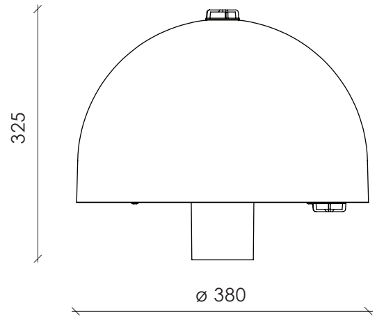
Dimensions with 2 Zhaga connectors
