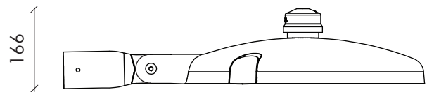
Dimensions with NEMA socket
