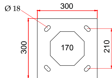
BASE PLATE
