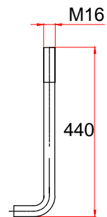
4 X M16 x 500 Anchor Bolts
