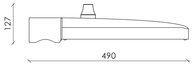
Dimensions with RF antenna
